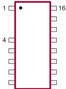
16-lead SOIC
