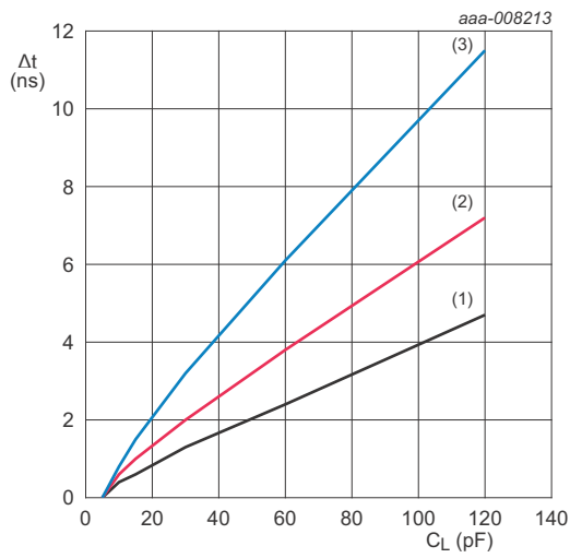
T_{amb} = -40\text{ °C to }+85\text{ °C unless otherwise specified.} (1) Minimum: V_{CC} = 1.6\text{ V} (2) Typical: T_{amb} = 25\text{ °C}; V_{CC} = 1.5\text{ V} (3) Maximum: V_{CC} = 1.4\text{ V}
