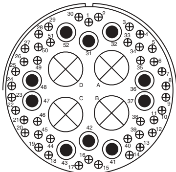
Insert Arrangement 48-51 Service Rating A Number of Contacts 42 10 4 Contact Size 16 8 0 (Coax) RG-41/U
