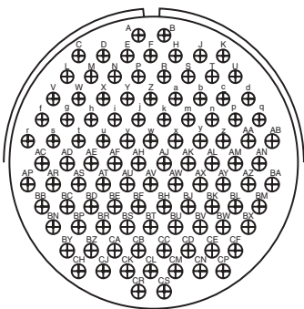
Insert Arrangement Service Rating Number of Contacts Contact Size 44-52 A 104 16
