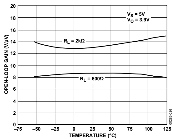
Figure 16. Open-Loop Gain vs. Temperature @ 5 V
