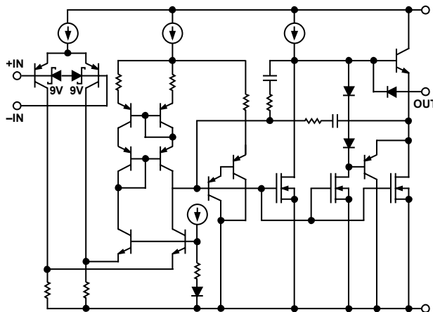
Figure 52. OP213 Simplified Schematic
