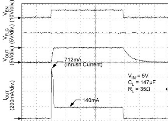
TIME (10ms/div.)
