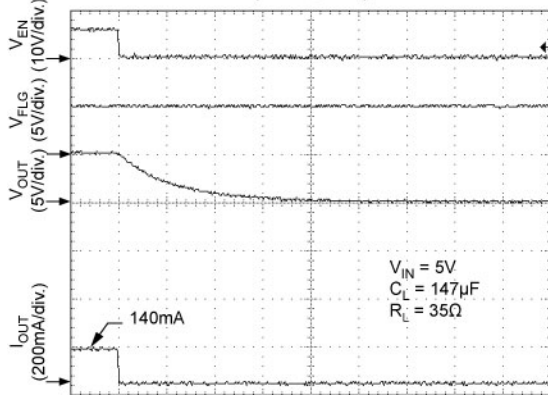
TIME (5ms/div.)
