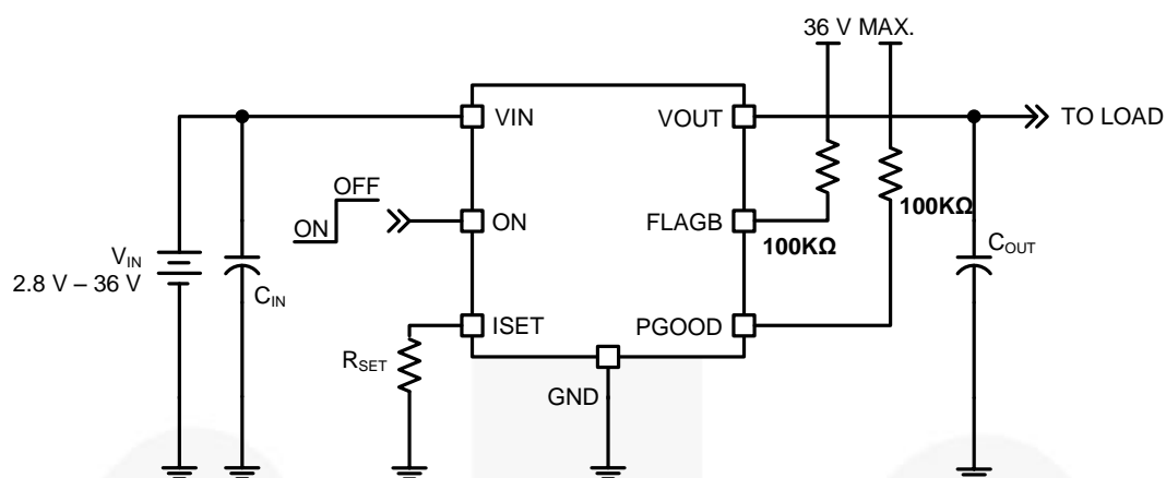
Figure 4. Typical Application
