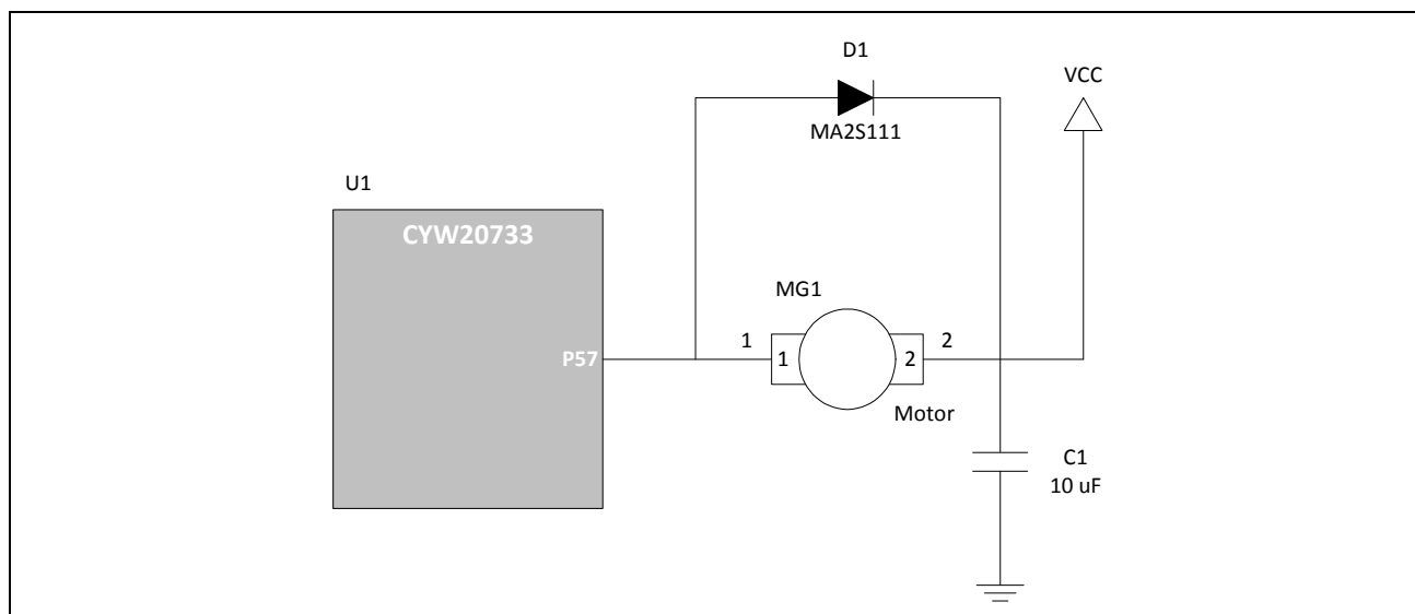
Figure 11. Motor/Vibrator Circuit
