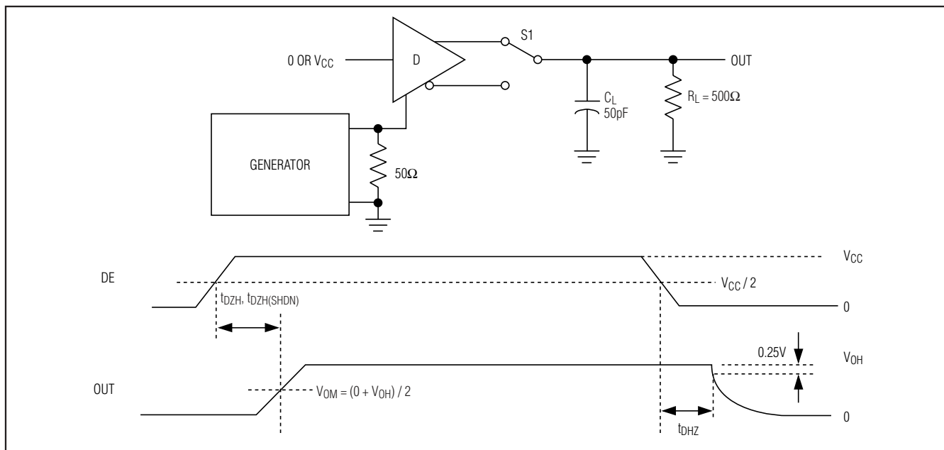
Figure 4. Driver Enable and Disable Times ( t_{DZH} , t_{DZH(SHDN)} , t_{DHL} , t_{DHL(SHDN)} )
