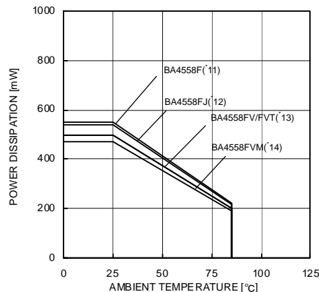
Fig. 50 Thermal resistance and derating curve
