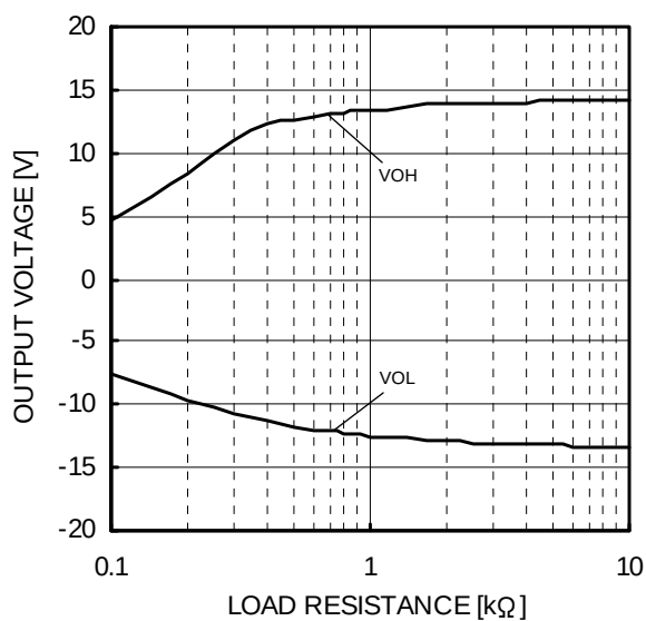
Fig.28 Maximum Output Voltage - Load Resistance ( V_{CC}/V_{EE}=+15V/-15V , T_a=25^\circ C )
