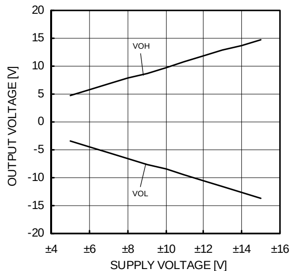
Fig.29 Maximum Output Voltage - Supply Voltage ( R_L=2k\Omega , T_a=25^\circ C )
