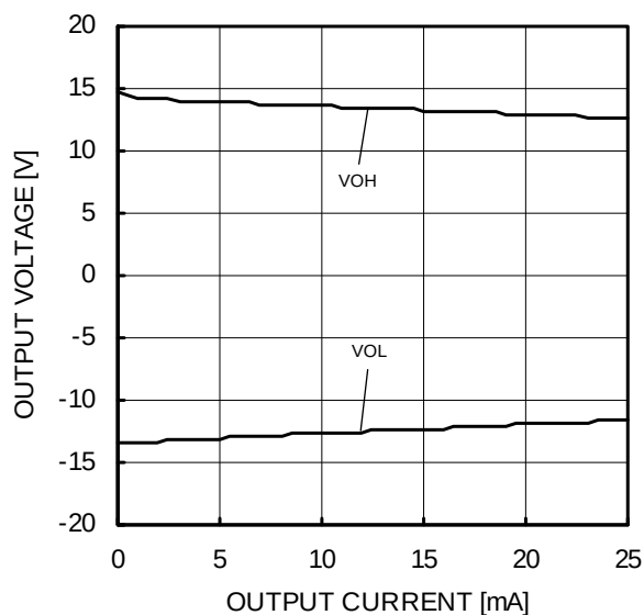
Fig.31 Maximum Output Voltage - Output Current ( V_{CC}/V_{EE}=+15V/-15V , T_a=25^\circ C )
