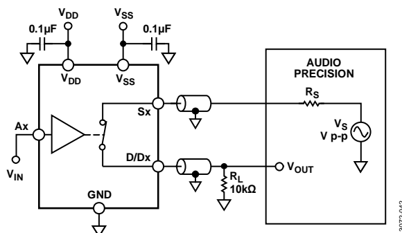
Figure 39. THD + N
