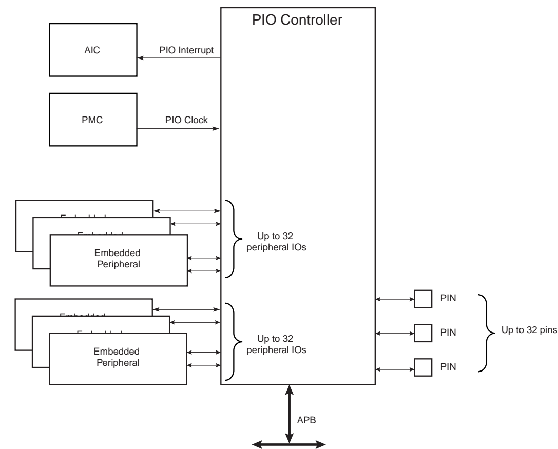
Figure 65. Block Diagram
