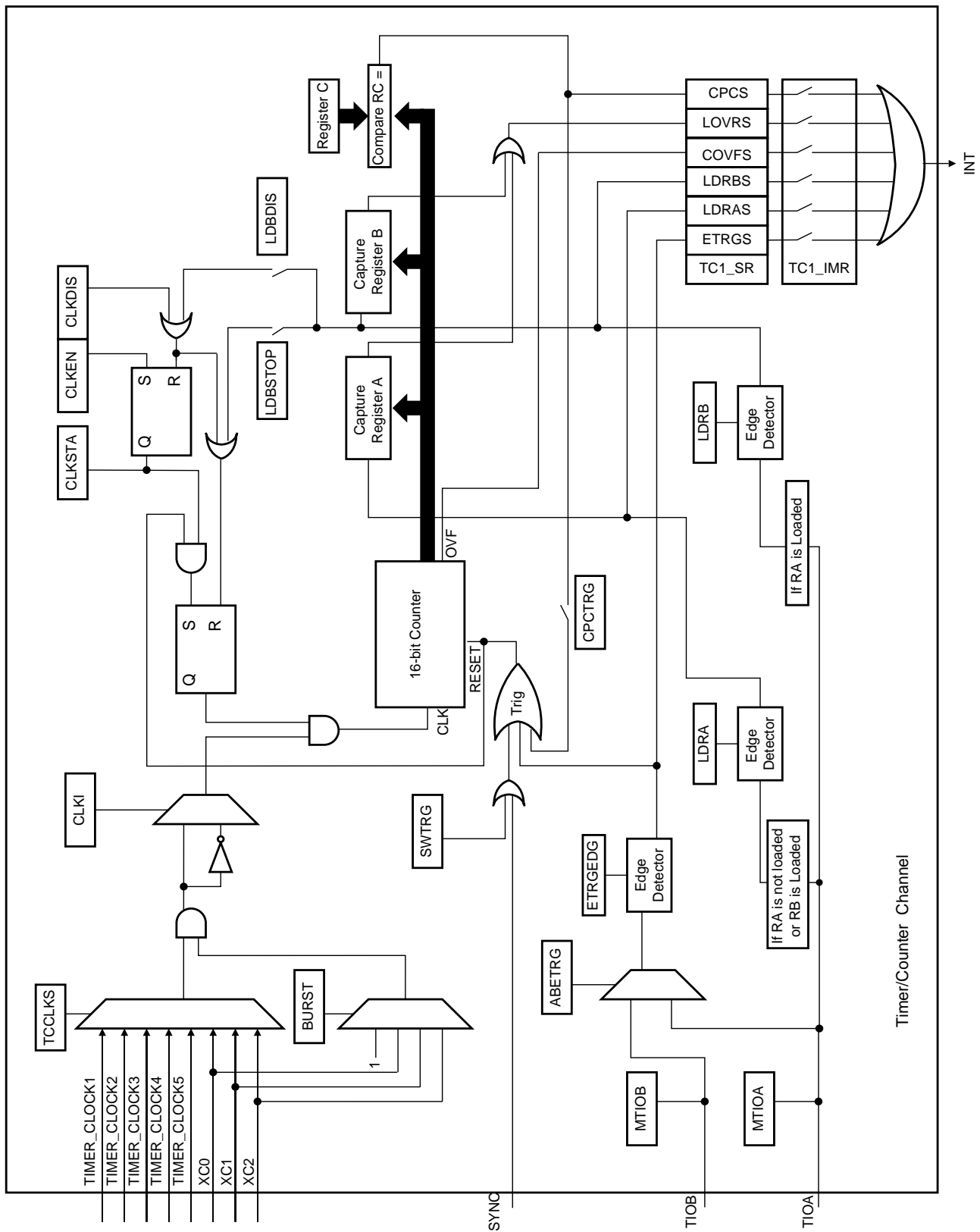
Figure 141. Capture Mode
