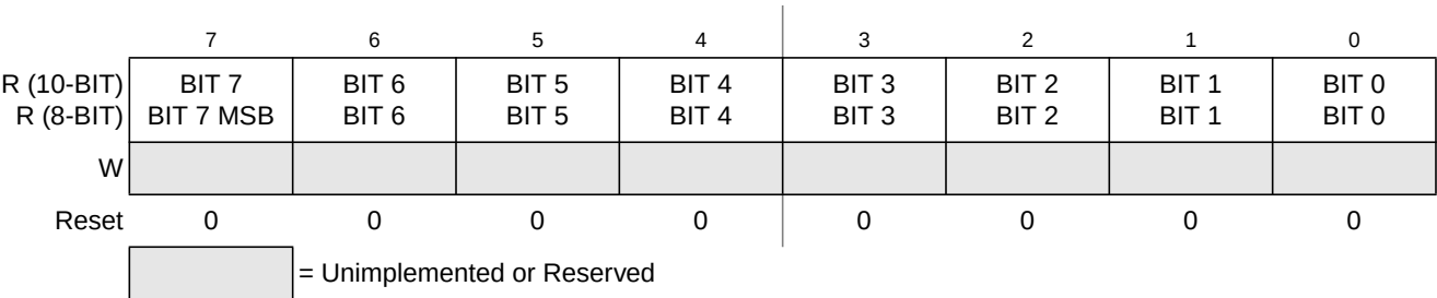
Figure 7-21. Right Justified, ATD Conversion Result Register x, Low Byte (ATDDRxL)
