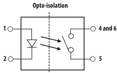
Equivalent Relay Diagram
