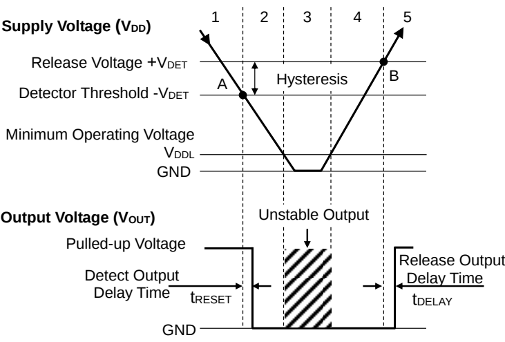
Operation Diagram
