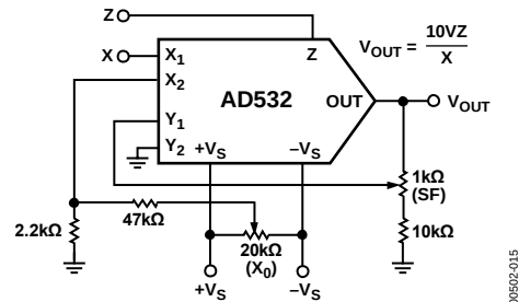
Figure 17. Divider Connection
