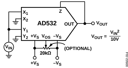
Figure 16. Squarer Connection
