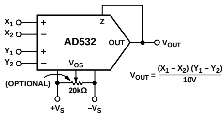
Figure 15. Multiplier Connection
