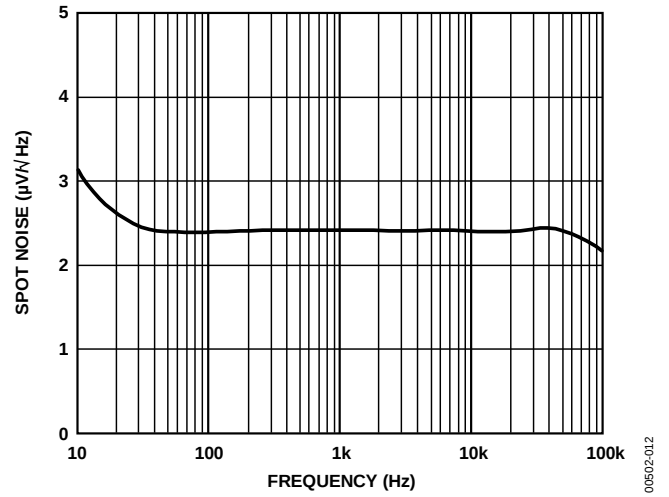
Figure 13. Spot Noise vs. Frequency
