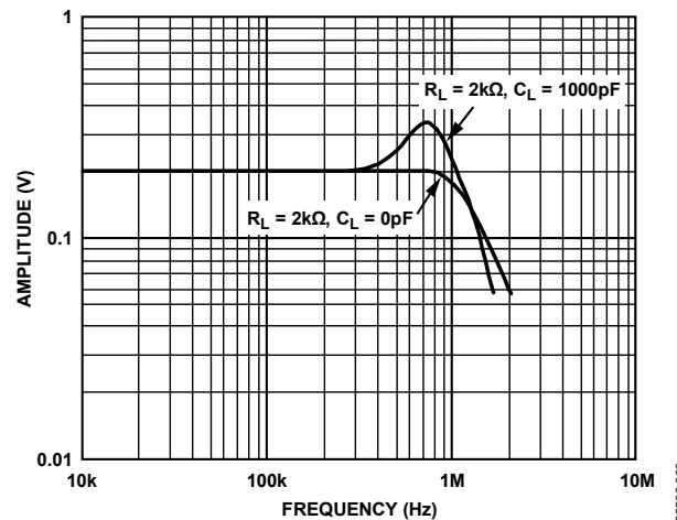
Figure 10. Frequency Response, Multiplying
