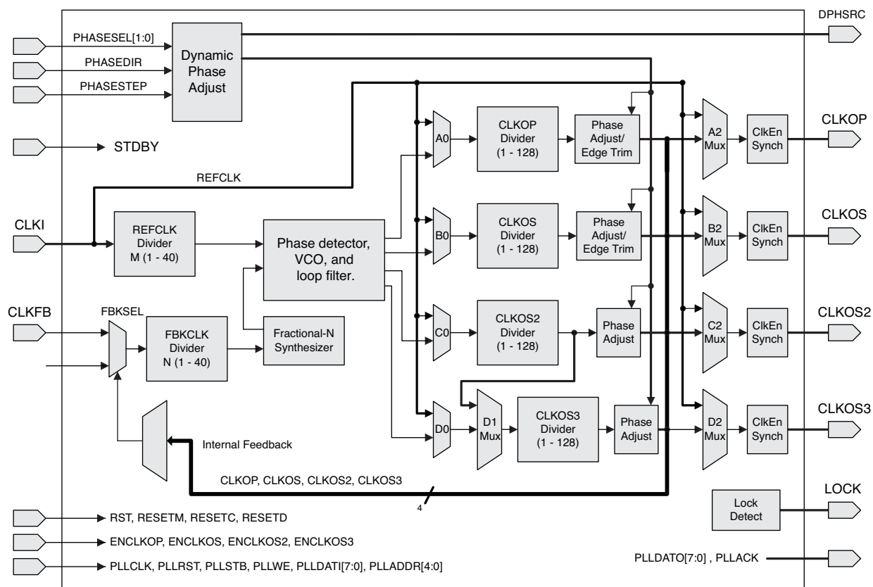
Figure 2-7. PLL Diagram
