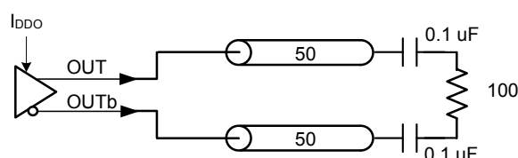
Differential Output Test Configuration
