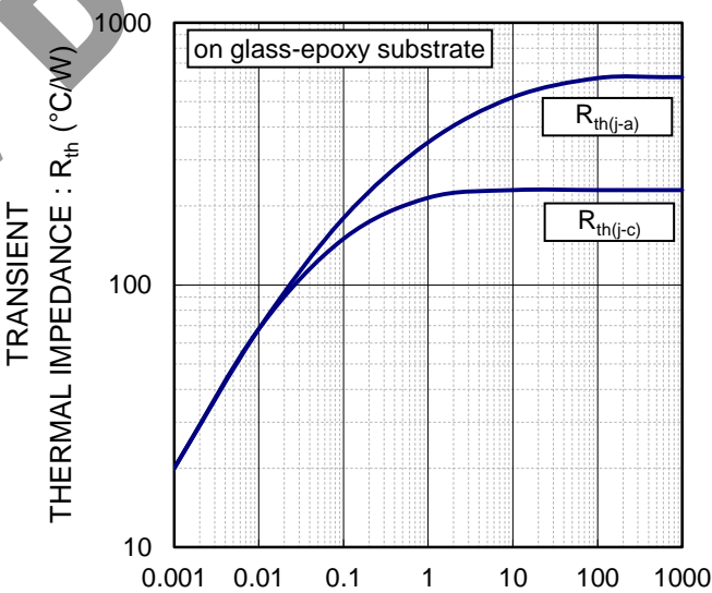
TIME : t (s) R_{th} - t CHARACTERISTICS
