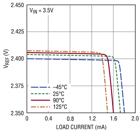
V_{REF} vs Load Current
