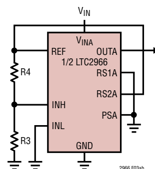
Figure 3b. Falling Edge Built-In Hysteresis by Grounding INL
