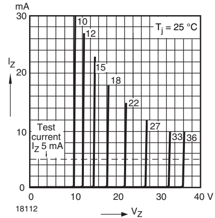
Fig. 15 - Breakdown Characteristics
