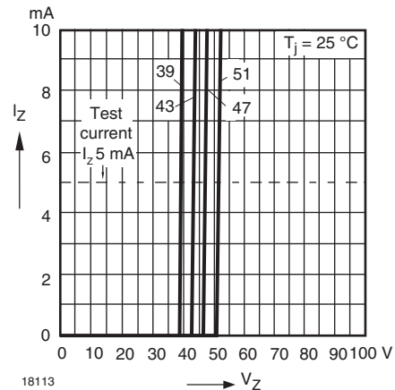
Fig. 16 - Breakdown Characteristics
