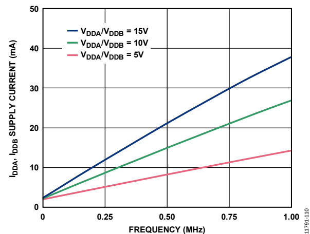
Figure 10. Typical I_{ODDA}, I_{ODDB} Supply Current vs. Frequency with 2 nF Load
