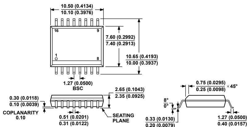
Dimensions shown in millimeters and (inches)
