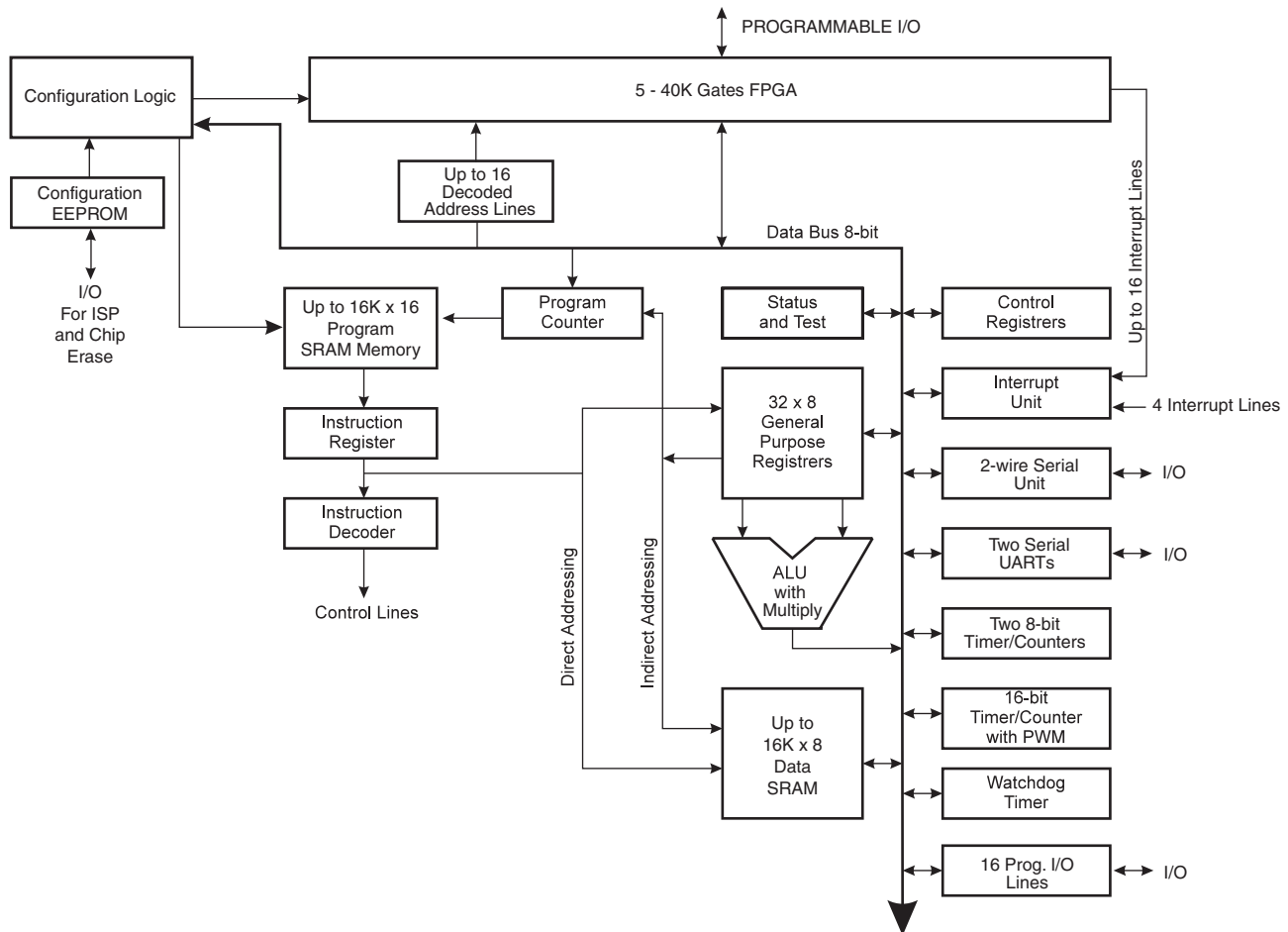
Figure 1-1. AT94S Architecture
