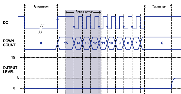
Figure 12. Preset Timing
