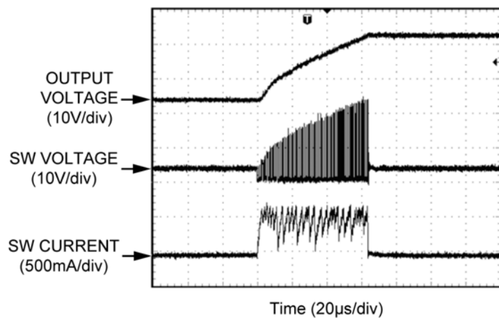
OVP Response
