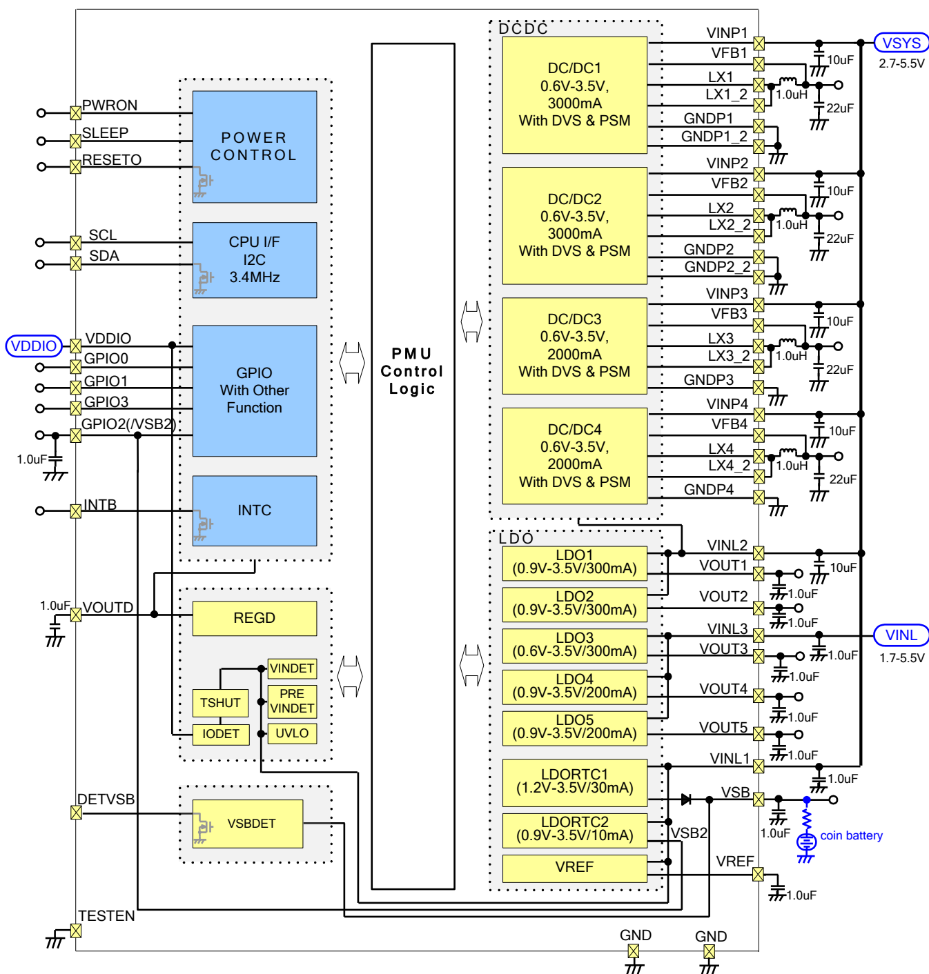
Fig 3-1 Block Diagram
