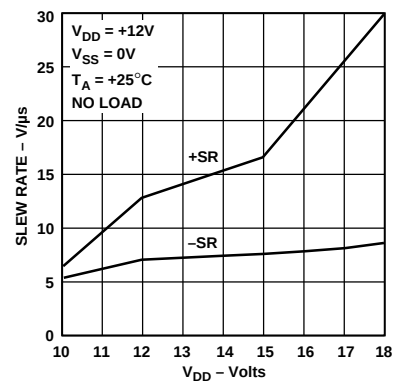
Slew Rate vs. V_{DD}
