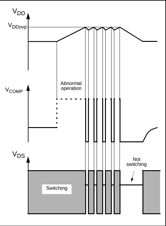
Figure 8. Overvoltage event
