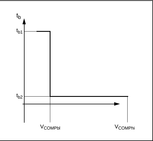
Figure 8. Overvoltage event
