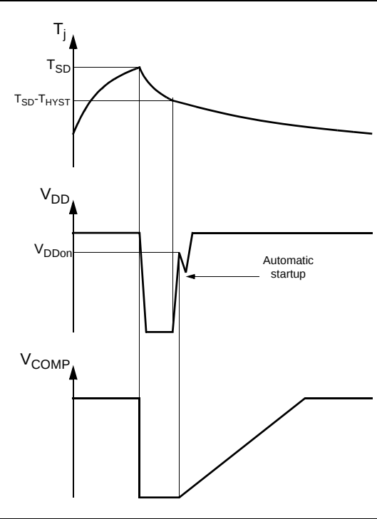
Figure 7. Thermal shutdown
