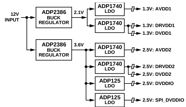
Figure 106. Power Supply Recommendation
