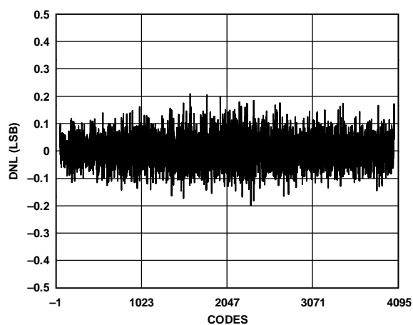
Figure 23. Differential Nonlinearity (DNL), \pm 0.2 LSB at 2.0 GSPS
