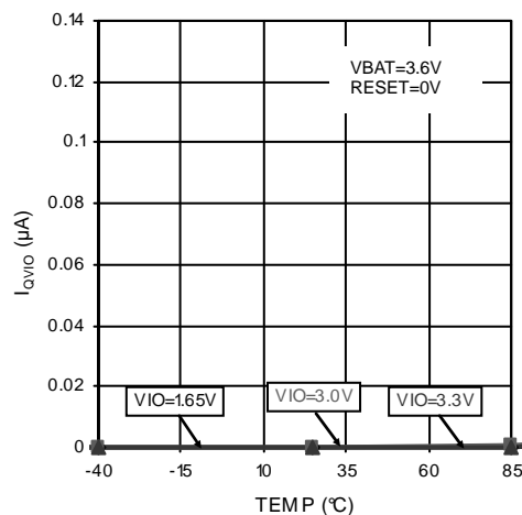
Figure 2. Quiescent Current (VIO) vs Temperature
