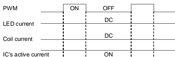
Figure 69. DC dimming
