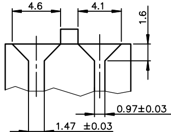
DETAIL-3: MATING SLOTS
