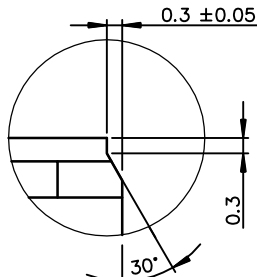
DETAIL-2: PIP CHAMFER SCALE 10/1
