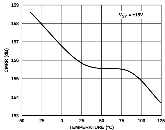
Figure 34. CMRR vs. Temperature
