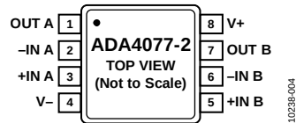
Figure 4. Pin Configuration, 8-Lead MSOP (RM Suffix)
