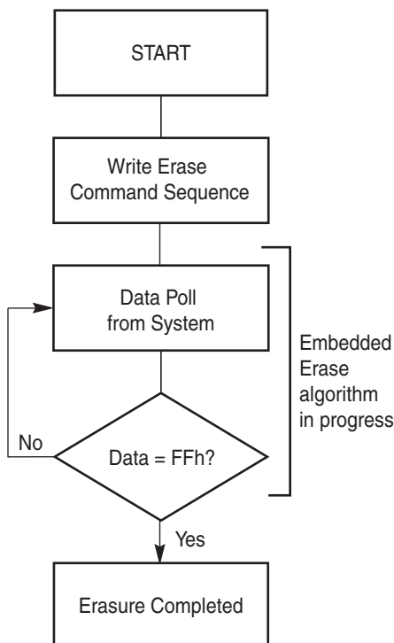
Figure 6. Erase Operation
