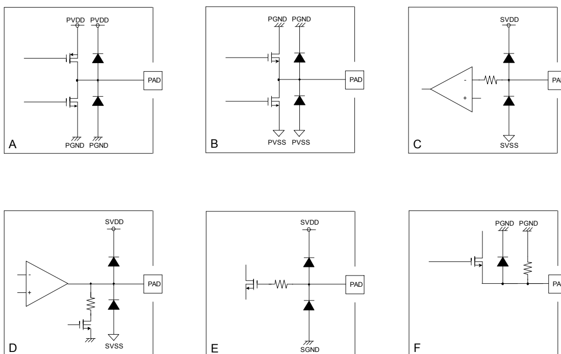
Fig.55 Pin equivalent circuit
