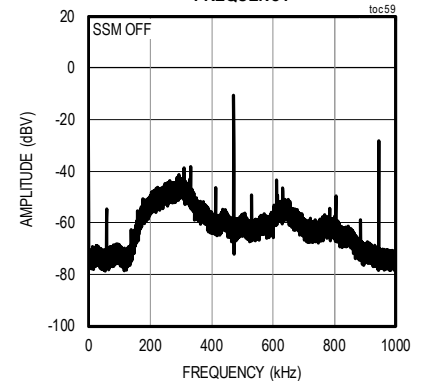
CLASS D OUTPUT FFT vs. FREQUENCY
