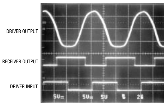
Figure 7. Driver Test Results at 250kbps
