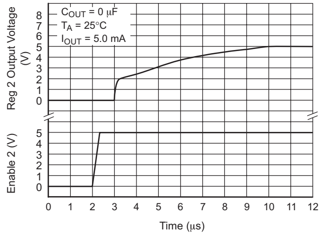
Figure 15. Regulator 2 Startup
