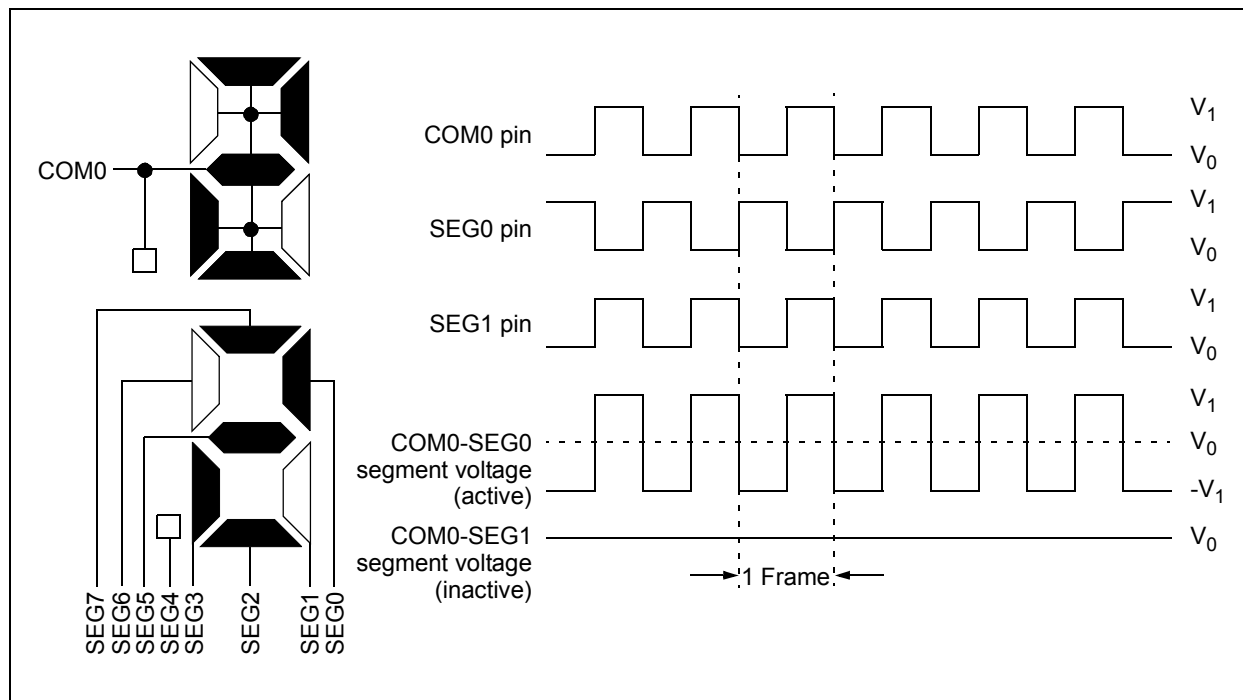
FIGURE 26-8: TYPE-A/TYPER-B WAVEFORMS IN STATIC DRIVE
