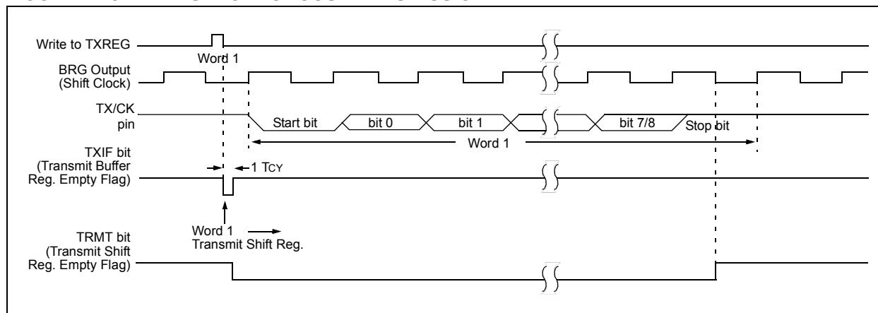
FIGURE 24-3: ASYNCHRONOUS TRANSMISSION
