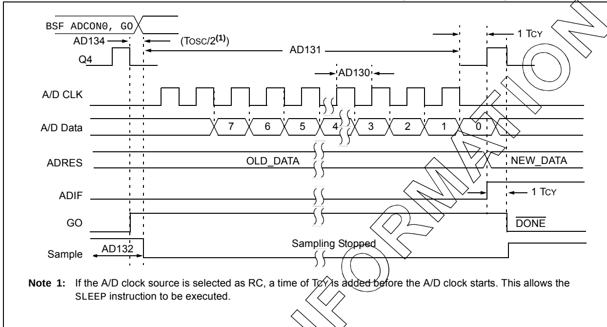
FIGURE 31-12: PIC16F/LF1938/39 A/D CONVERSION TIMING (NORMAL MODE)
