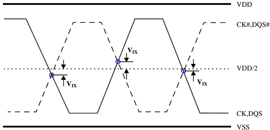
Figure 4.4. V_{IX} Definition
