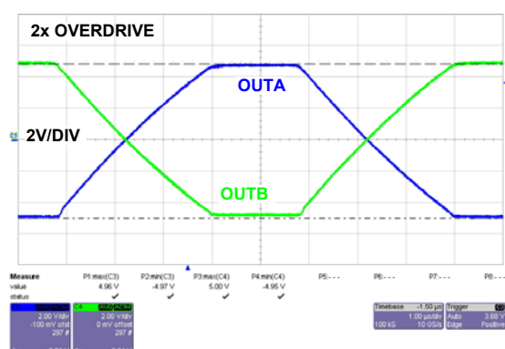
FIGURE 30. OVERDRIVE RECOVERY
