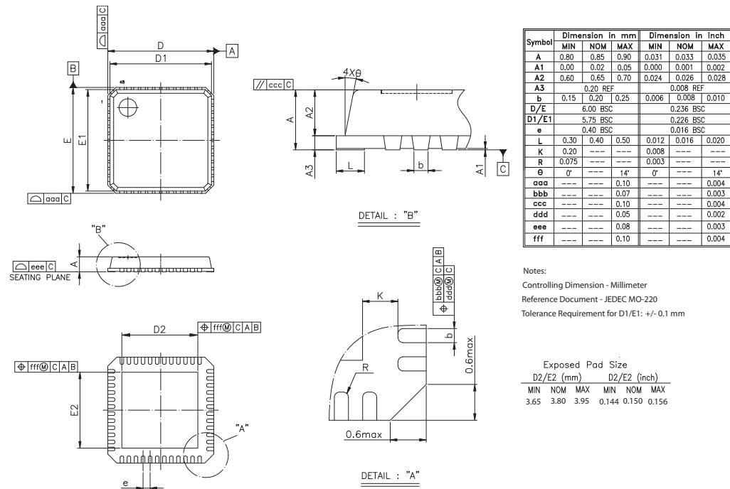
Figure 3. Package Dimensions
