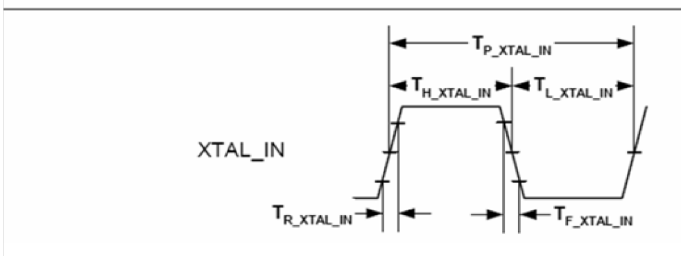
Figure 22. XTAL Timing Diagram
