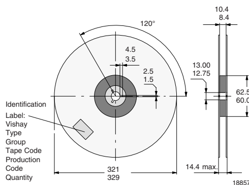
Figure 25. Reel dimensions - GS18
