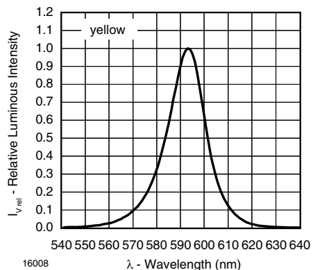
Figure 19. Relative Intensity vs. Wavelength
