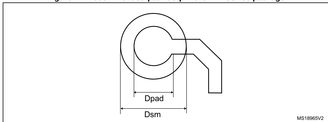
Figure 47. Recommended pad footprint for WLCSP36 package
