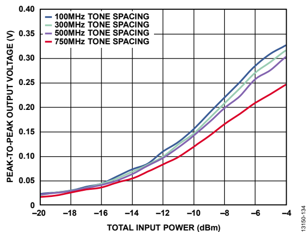
Figure 34. Envelope Detector Peak-to-Peak Output Voltage vs. Total Input Power at Various Tone Spacings, R_F = 71 GHz, V_{CTL1}/V_{CTL2} = -5 V, V_{DET} = 4 V with 150\ \Omega Load Impedance at ENV_{DET}
